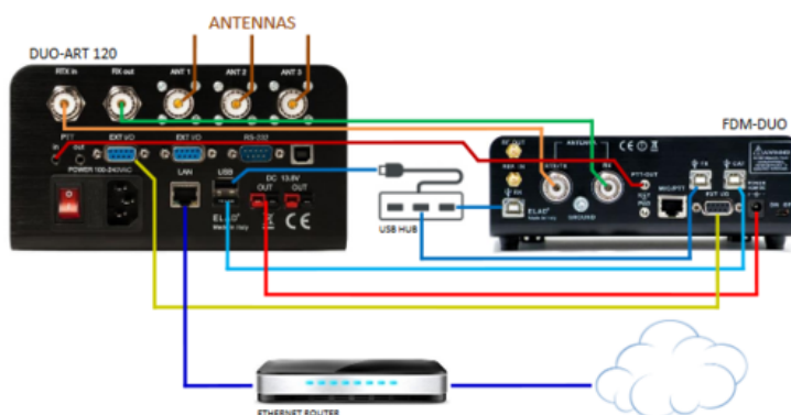
FDM DUO / DUO ART connection schematics as per DUO ART Manual
