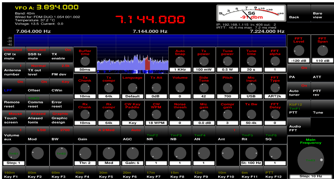
Settings screen
